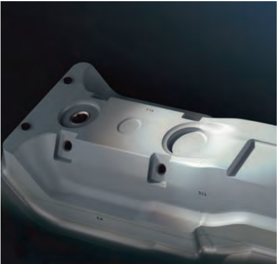
Gauge with high dimensional accuracy milled out of SikaBlock® M1050
