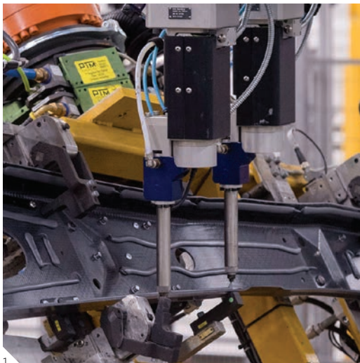
1 SikaPower® MBX - Central tunnel bonding (CFRP - steel)
