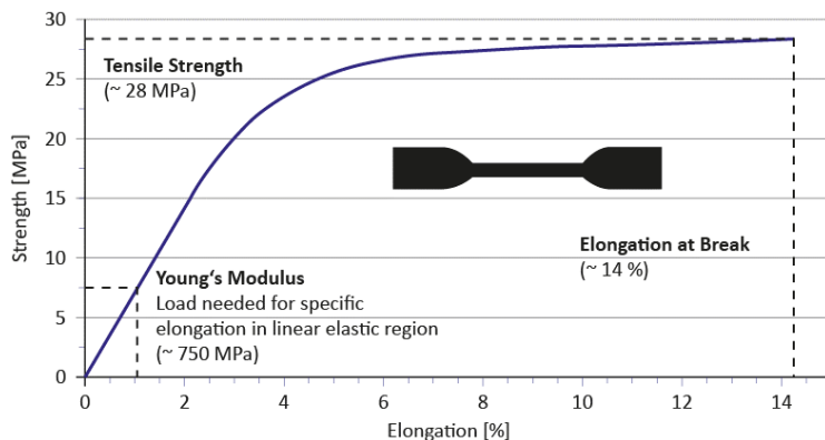
Diagram 7: Dumbbell specimen for tensile testing, technical stress-strain curve
