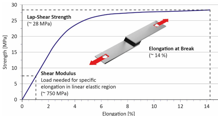
Figure 7: Illustration of single lap joint specimen and results
