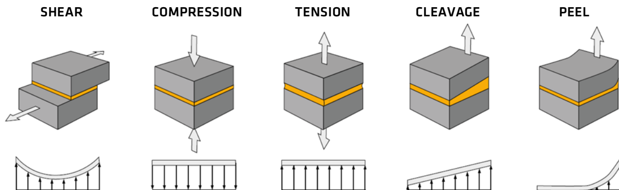
Figure 15: Loaded joints and stress distribution
