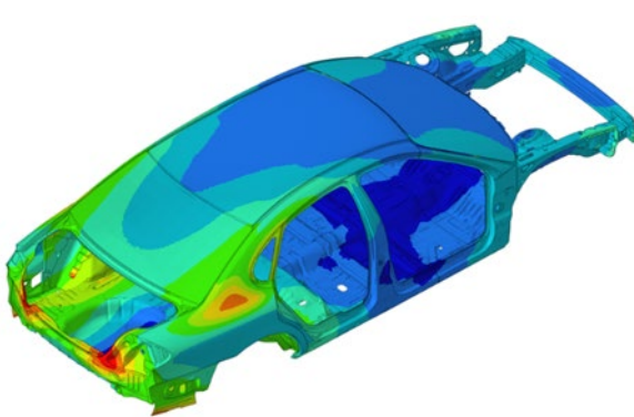
Figure 25: Global bending Eigenform of car body (displacement magnitude, quantitative)
